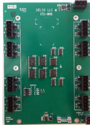
CN-SLX-170-IN16 Input Expansion Board with 16 supervised inputs
