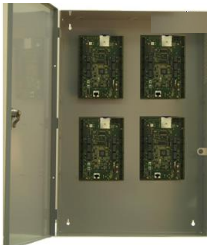
Large enclosure fits four 1700s or combination or four 170 I/O boards
